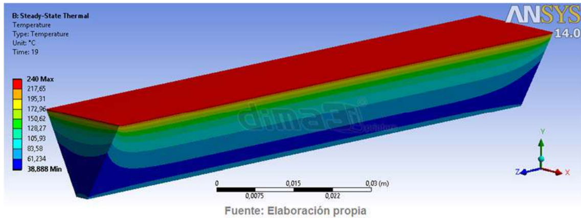
Figure 7. Thermal gradient with bed at 80°C (176°F)
